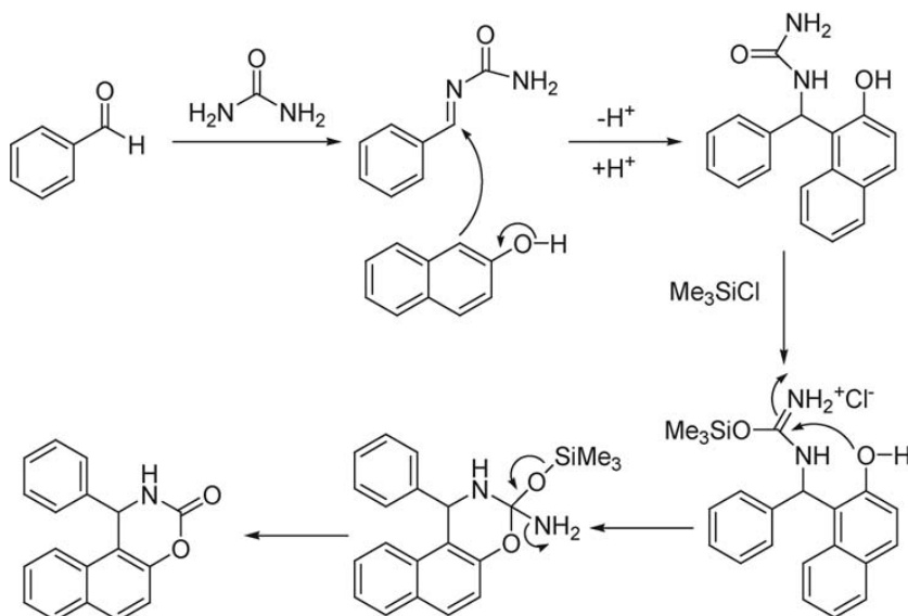
Scheme 2 Plausible reaction mechanism.
