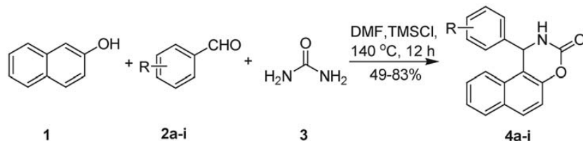
Scheme 1 One-pot reaction of 2-naphthol, aromatic aldehydes and urea promoted by TMSCl.
